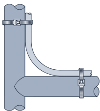
Fixing of cables right
